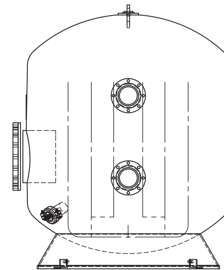
INTERNAL PLUMBING VIEW
